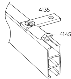
ceiling mounting with ceiling bracket 4135 and dust cover 4145 to seal the gap
