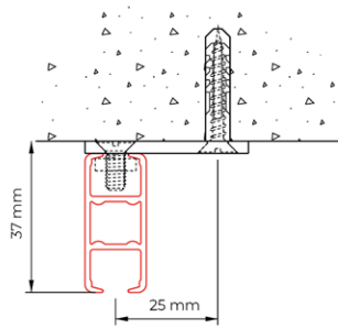
ceiling mounting with ceiling bracket 4135
