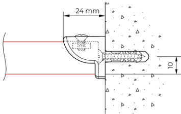
wall mounting 4200 with wall bracket 4249
