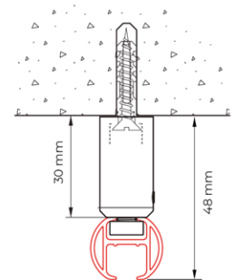
ceiling mounting 4200 with suspension hanger
