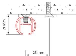
ceiling mounting 4200 with ceiling bracket 5153
