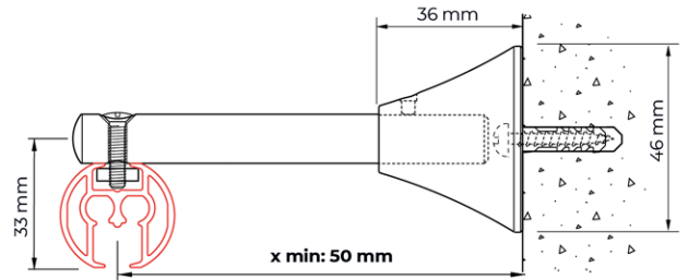
wall mounting 5100 with adaptable extension bracket 4217-101, bracket can be cut back to x=50mm.
